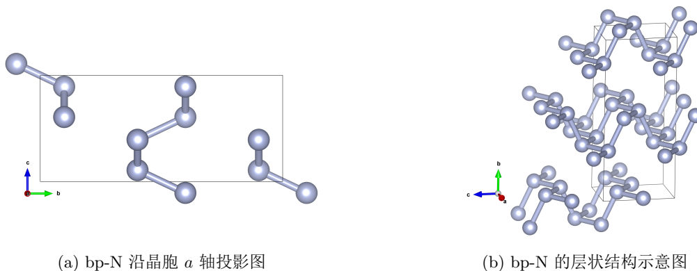
图 3: bp-N 的晶体结构 Cmce a = 213.43 \text{ pm} , b = 653.42 \text{ pm} , c = 285.99 \text{ pm}
